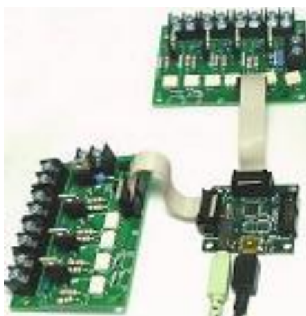
Fig 1. Connection 2 Triac Module to Base Module
