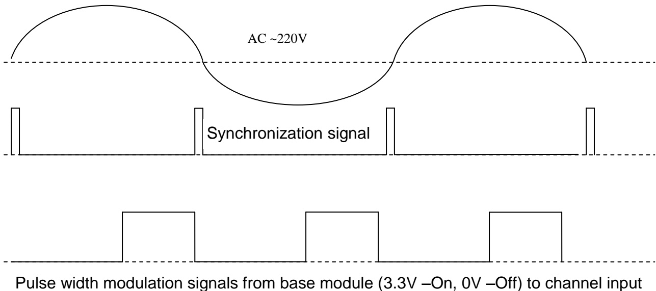
Fig 5. Synchronization signal:
