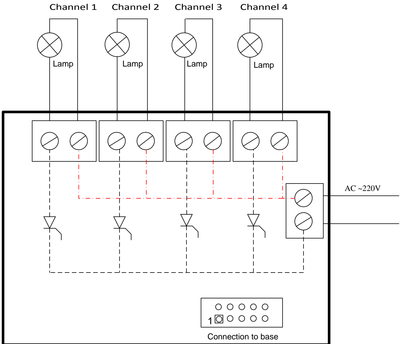
Fig 2. Block diagram Triac Module
